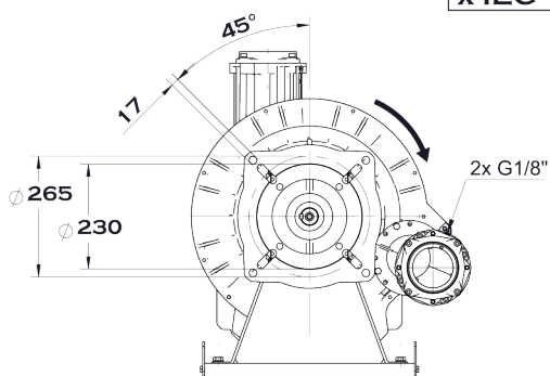
x IEC 132-B5
